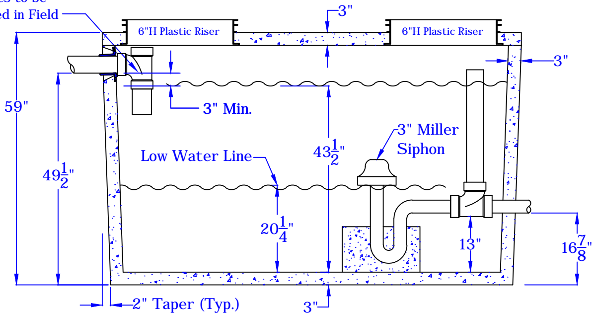
AA Section of 1000 Gallon Siphon Tank No Scale
