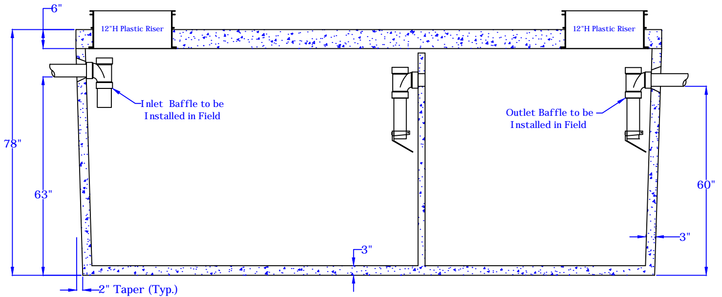
Section of 2500 Gallon 2 Compartment Tank No Scale
