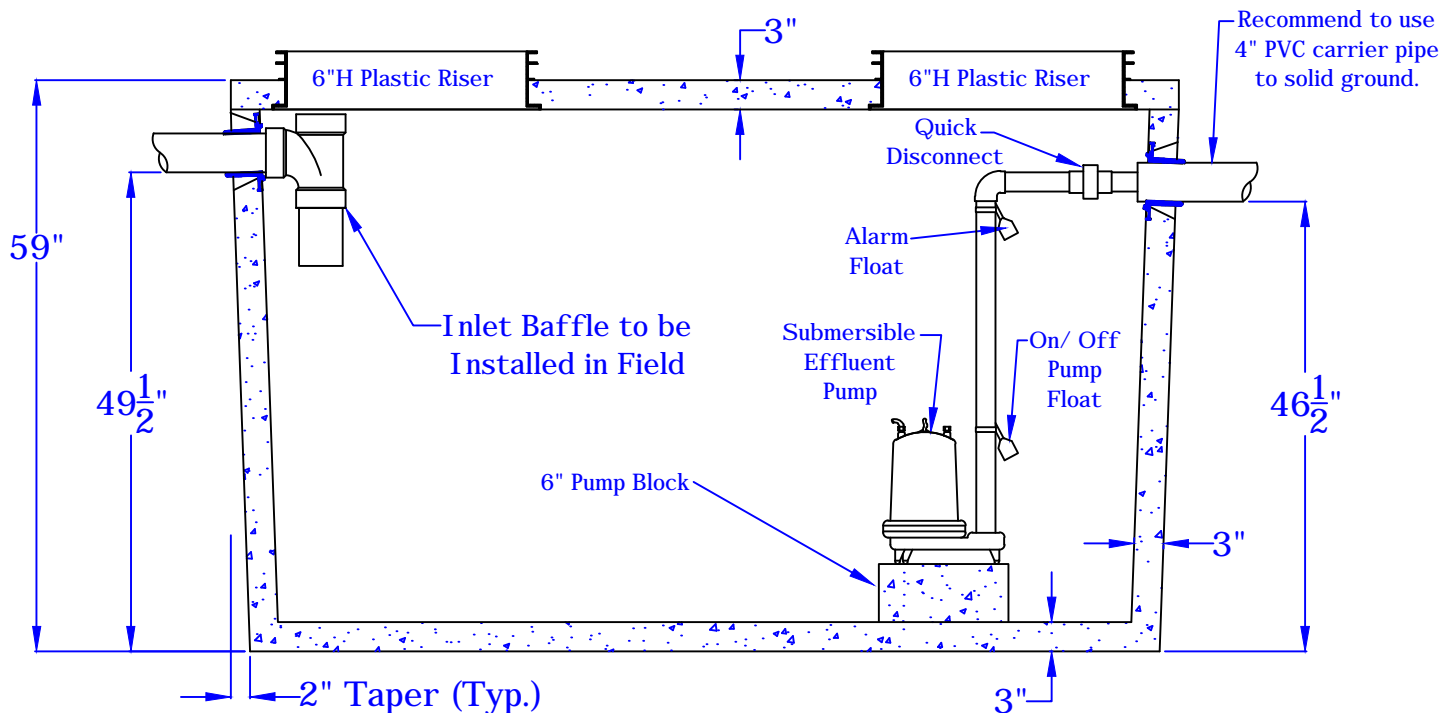
AA Section of 1000 Gallon Dose Tank No Scale
