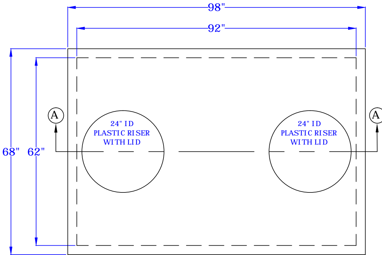
Plan View of Lid
