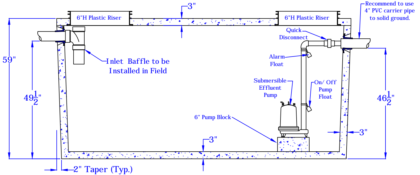
AA Section of 1250 Gallon Dose Tank No Scale
