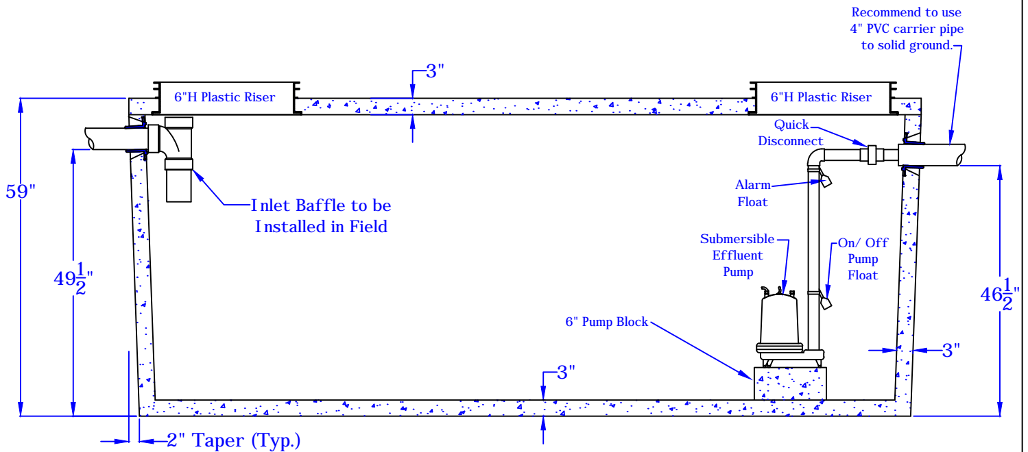
AA Section of 1500 Gallon Dose Tank No Scale
