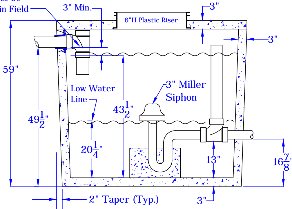
AA Section of 500 Gallon Siphon Tank No Scale
