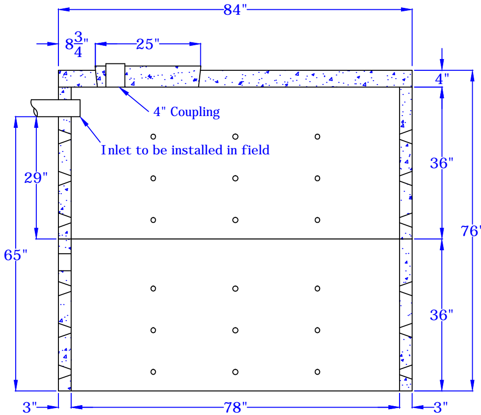
AA Section of 1400 Gallon Drywell No Scale
