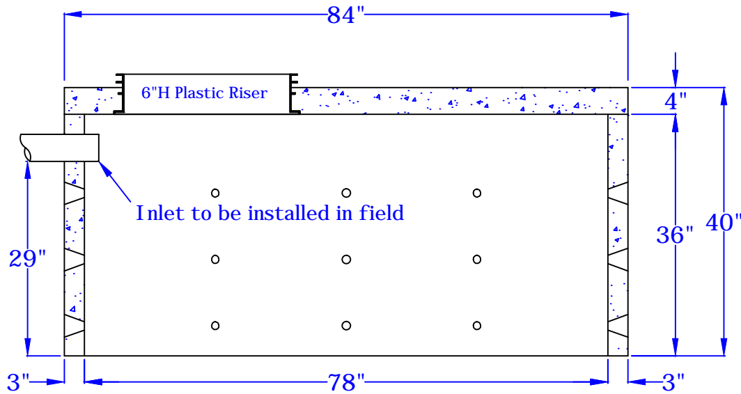
AA Section of 700 Gallon Dry Well No Scale
