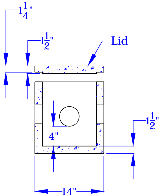
BB Section Of Distribution Box No Scale
