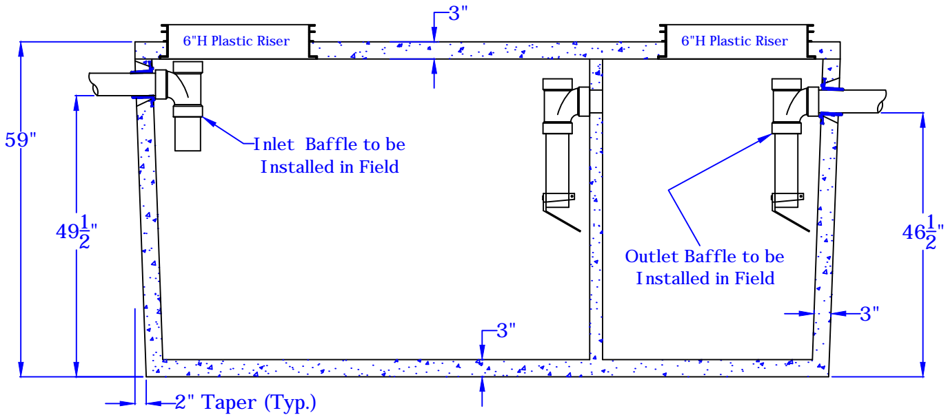
Section AA of 1250 Gallon 2 Compartment Septic Tank No Scale
