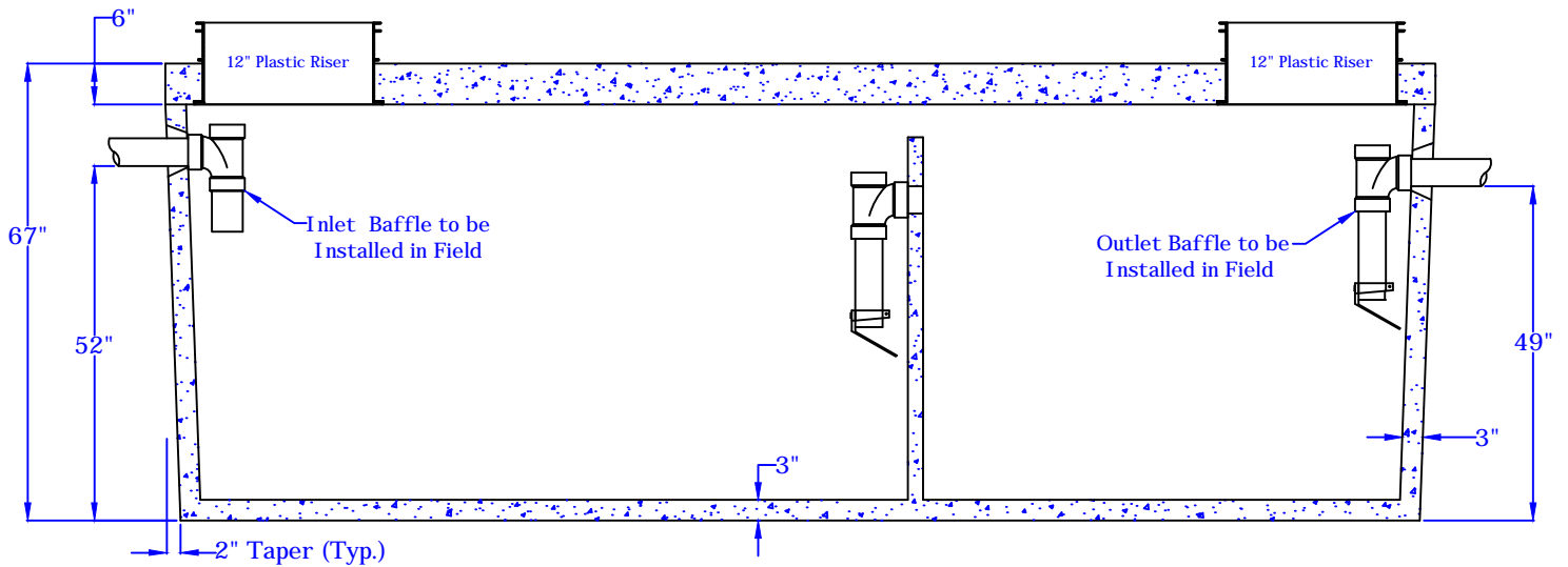
AA Section of 2000 Gallon 2 Compartment Tank No Scale
