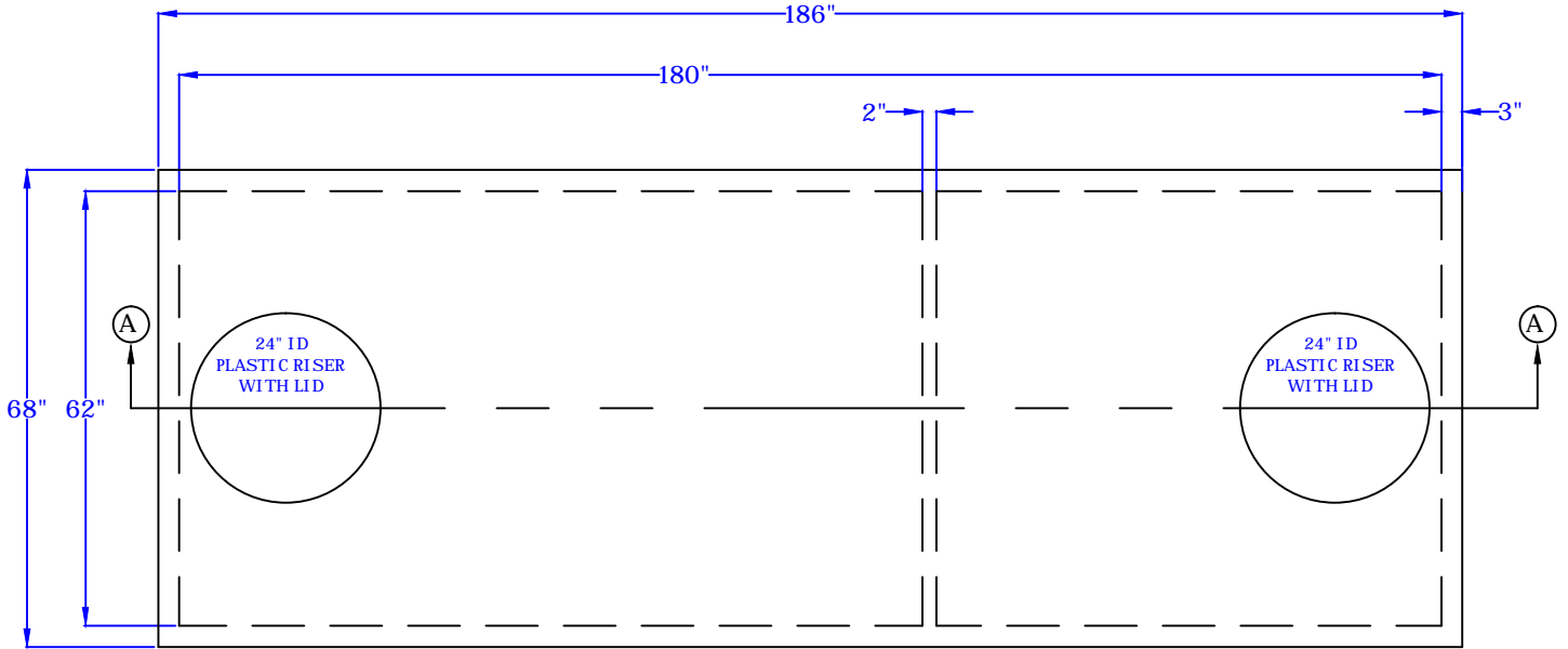
Plan View of Lid No Scale
